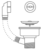
Ref. W90/O 90mm Basket Strainer Waste & Overflow Chrome: £21 Brushed Steel: £31 Gold: £38
