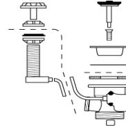
Ref. WPU90 90mm Pop-up Basket Strainer Waste Chrome: £32 Brushed Steel: £46
